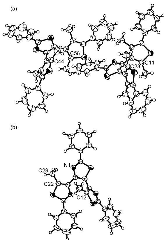
Figure 3. ORTEP drawings of open-ring isomer in crystal 1a (a) and in crystal 2a (b), showing 50% probability displacement ellipsoids. Two different alternately packed conformations existed for 1a in the single-crystalline phase.
