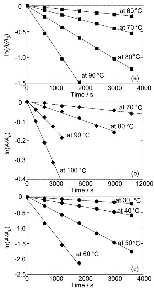
Figure 4. Decay lines of peak absorbance by thermal cycloreversion reactions of 1b (a), 2b (b), and 4b (c) at various temperatures in toluene.
