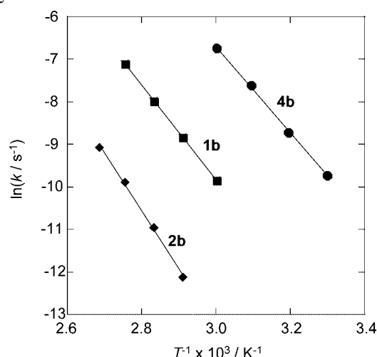
Figure 5. Temperature dependence of the thermal fading rates of 1b , 2b , and 4b in toluene.
