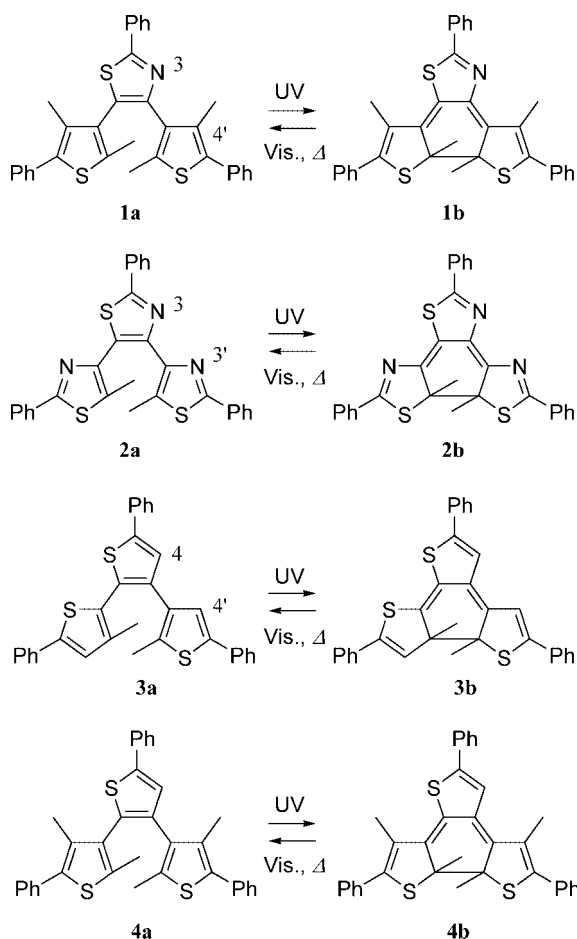
Scheme 1. Photochemical and thermal interconversion of terarylenes 1 – 4 .
