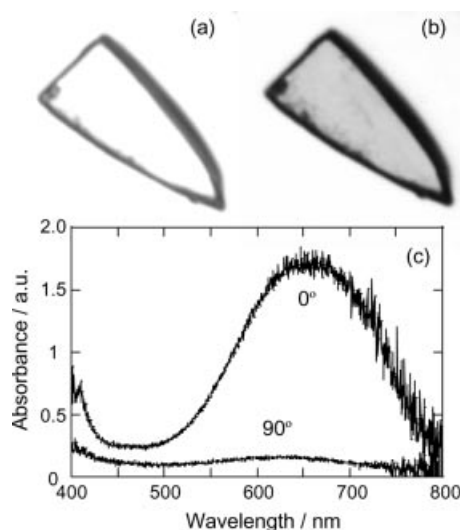
Figure 2. Photographs of crystal 1 before (a) and after (b) irradiation with UV light. c) Polarized absorption spectra of the photo-generated blue crystal of 1 .
