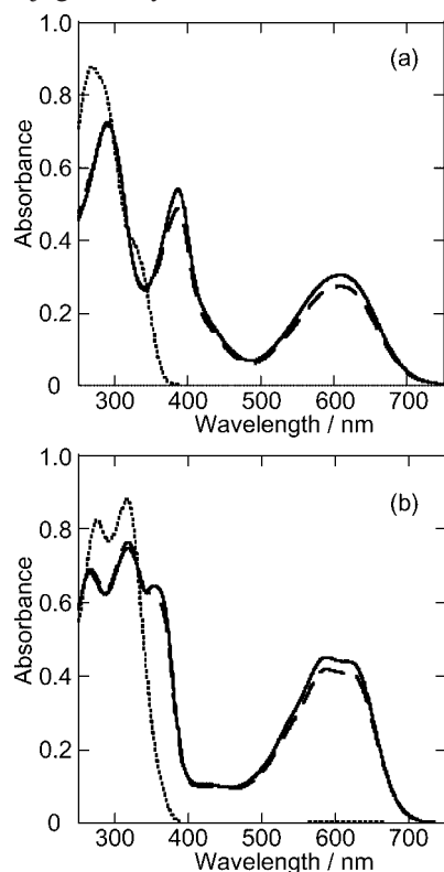
Figure 1. Absorption spectral changes of 1 (a) and 2 (b) in hexane: open-form a (dotted lines), closed-form b (solid lines) and photo-stationary state under irradiation with 313 nm light (dashed lines). The concentrations of 1 and 2 were 2.5 \times 10^{-5} and 2.9 \times 10^{-5} M, respectively.
