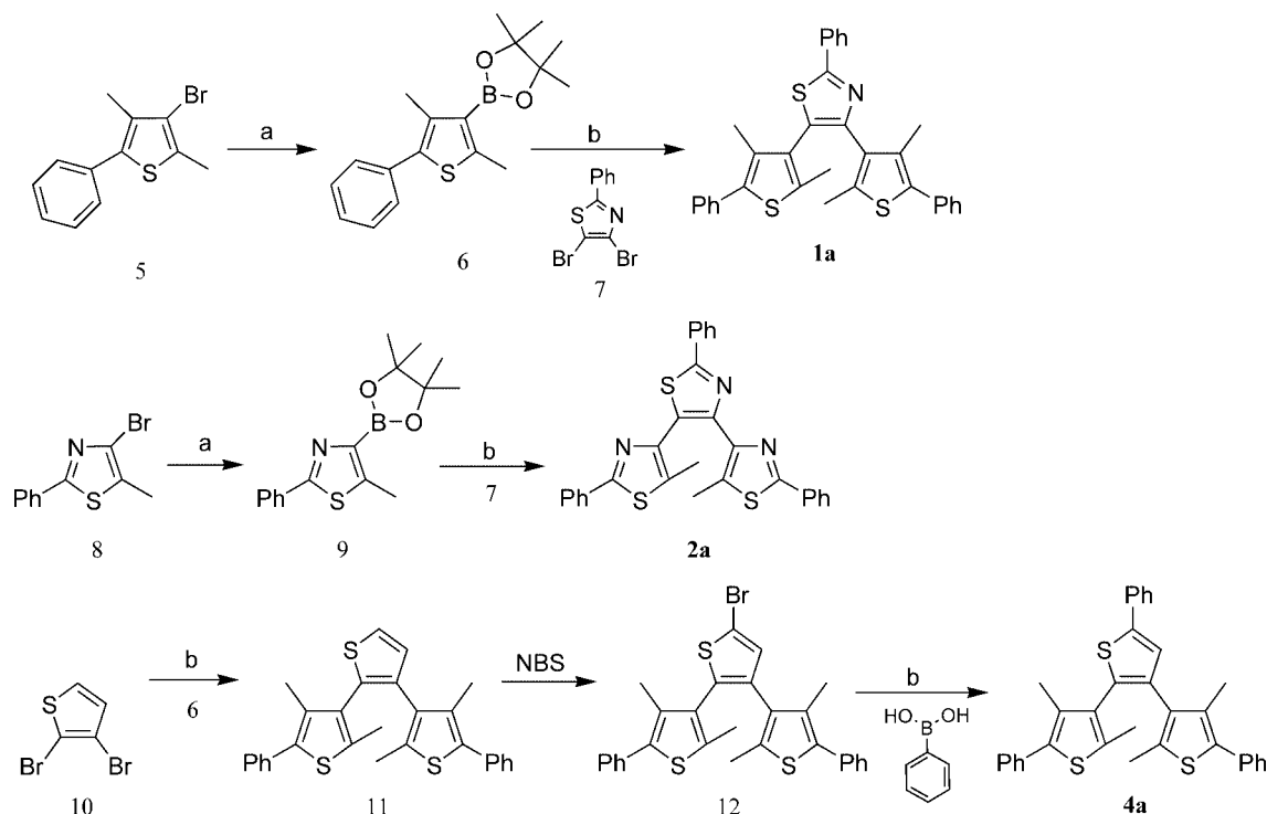
Scheme 2. Synthesis of photochromic terarylenes 1a , 2a , and 4a . Conditions: a; 1) n BuLi, 2) 2-isopropoxy-4,4,5,5-tetramethyl-1,3,2-dioxaborolane. b; K_3PO_4 , Pd(PPh_3)_4/H_2O , 1,4-dioxane.
